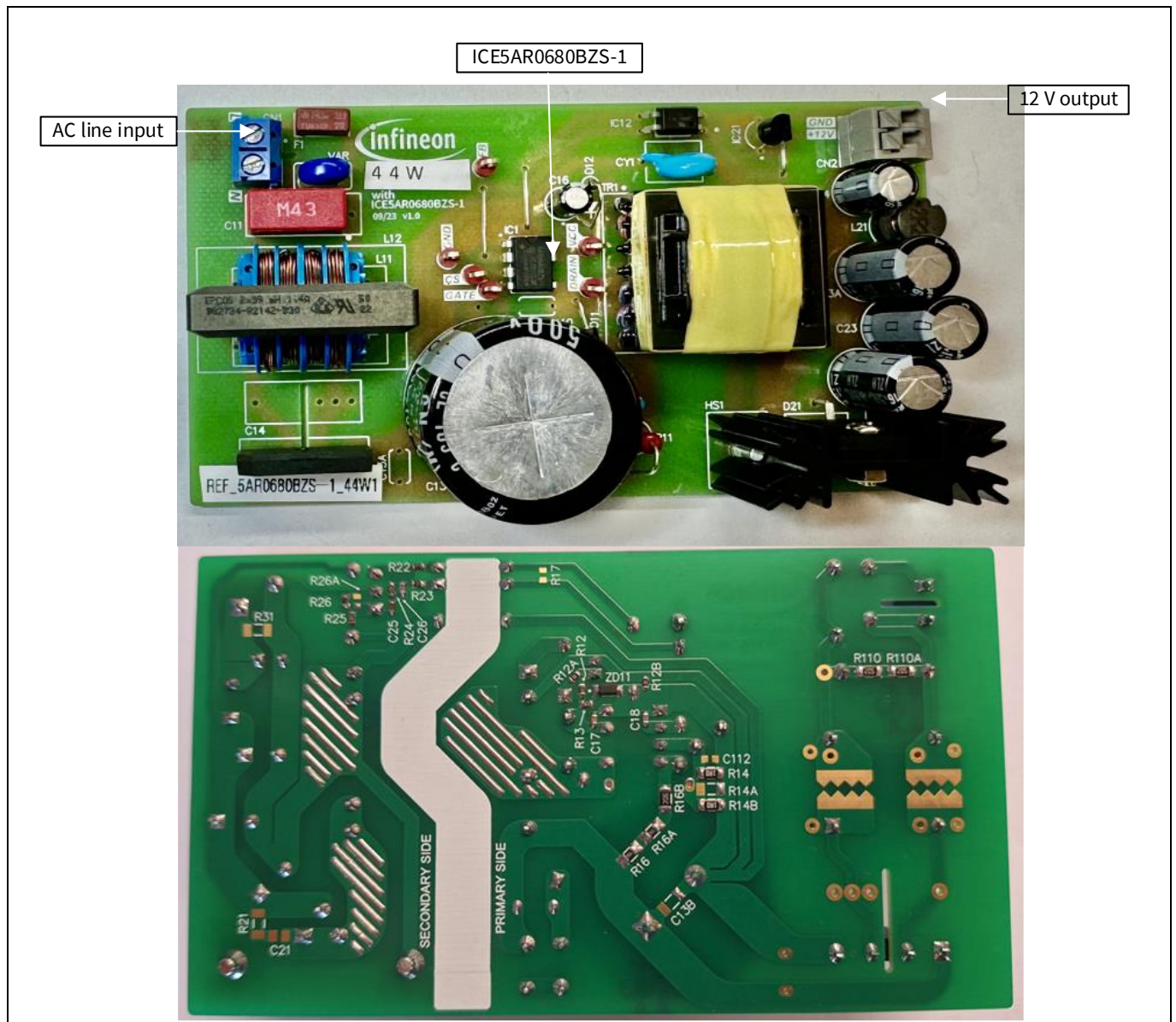
Figure 1 REF_5AR0680BZS-1_44W1
