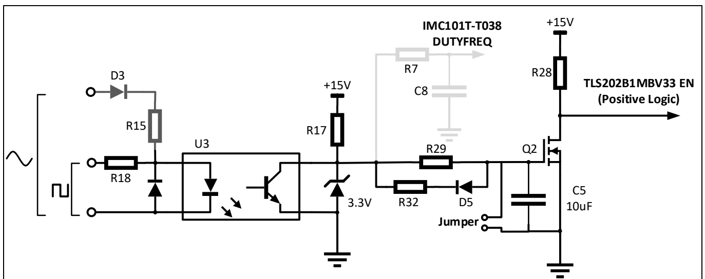
Figure 25 TLS202B1MBV33 Enable function control circuit
