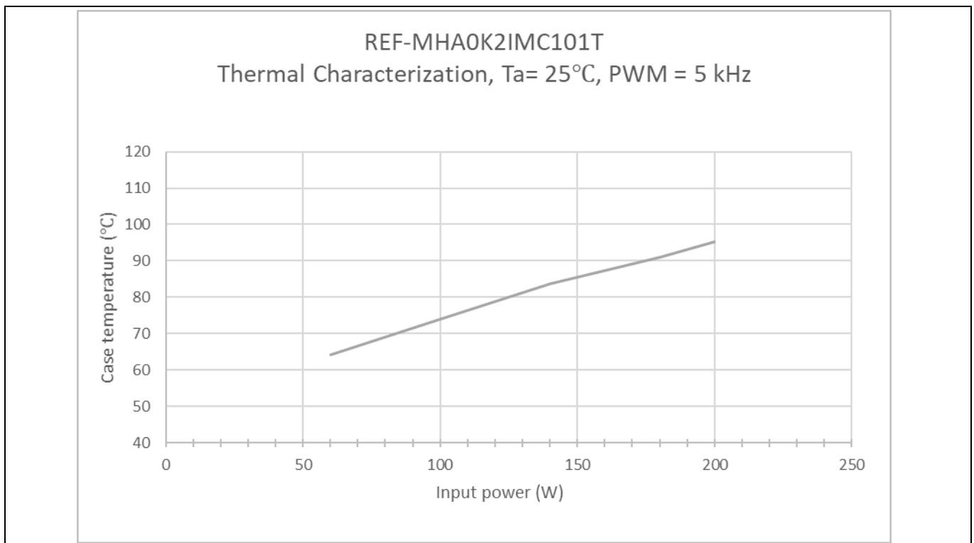
Figure 28 REF-MHA0K2IMC101T thermal characterization case temperature - input power, t_{amb} = 25^{\circ}\text{C}
