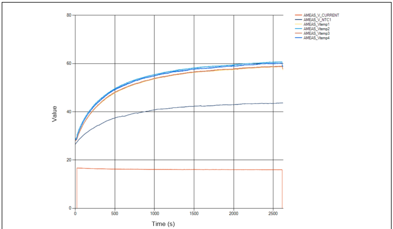
Figure 33 16 A DC continuous current
