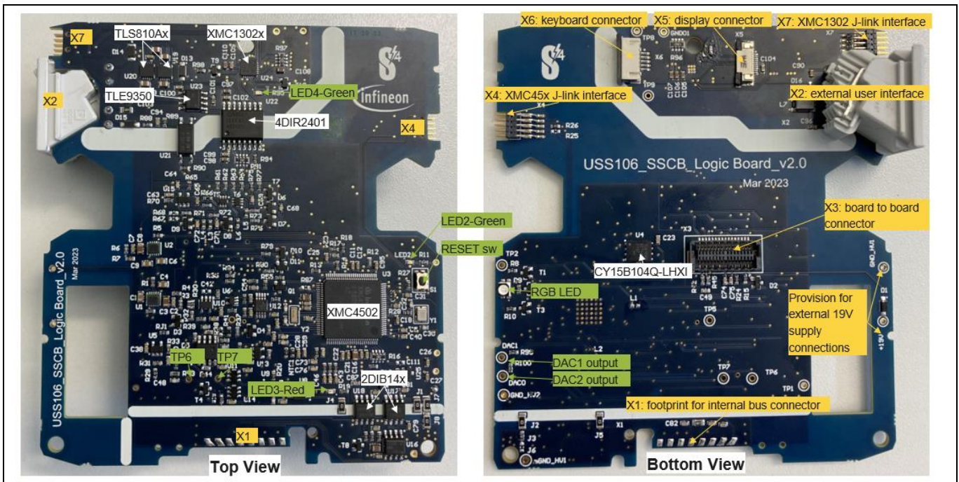
Figure 9 Logic board
