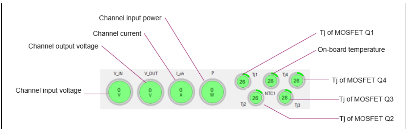
Figure 16 GUI temperature, current, and voltage indicators
