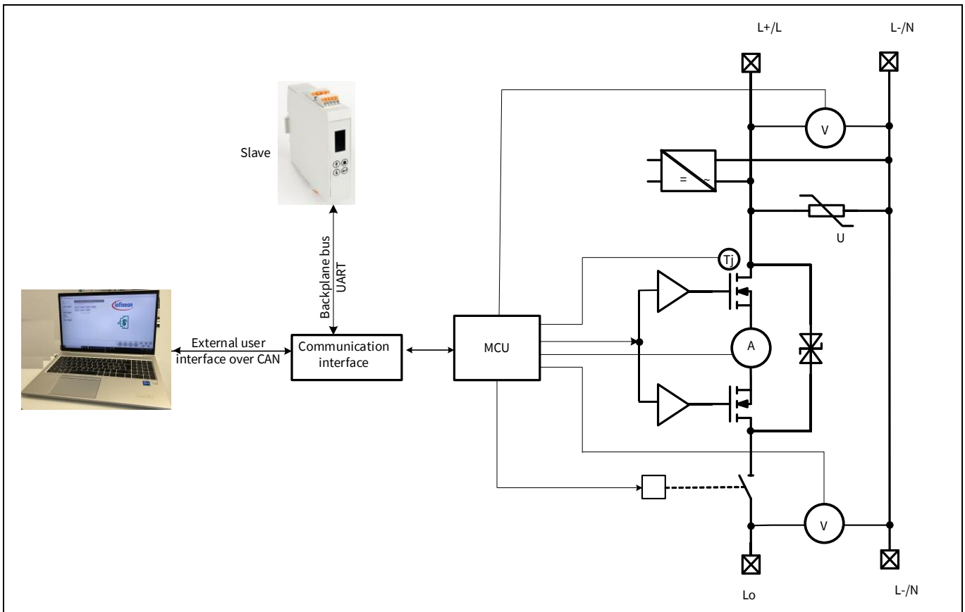
Figure 6 Block scheme
