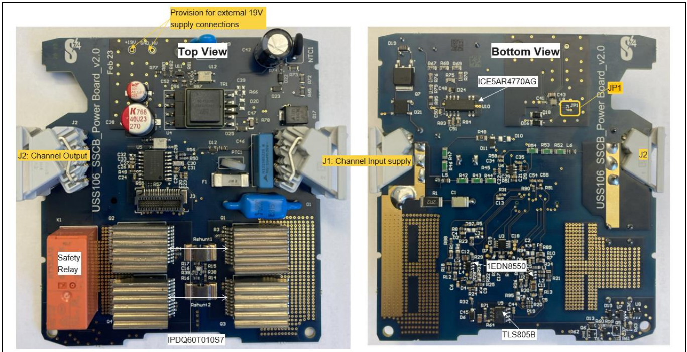
Figure 8 Power board
