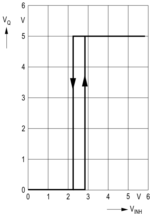
Output voltage V_Q versus inhibit voltage V_{INH}
