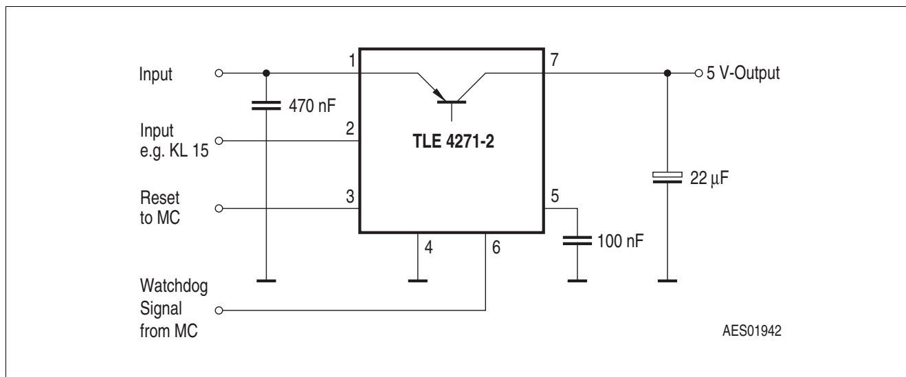
Figure 4 Circuit
