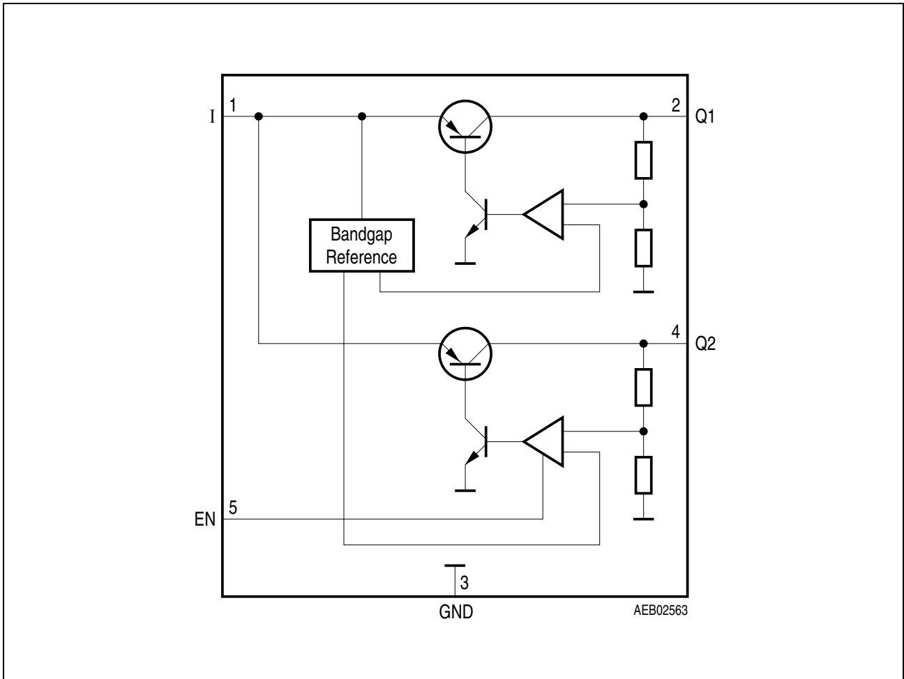
Figure 2 Block Diagram
