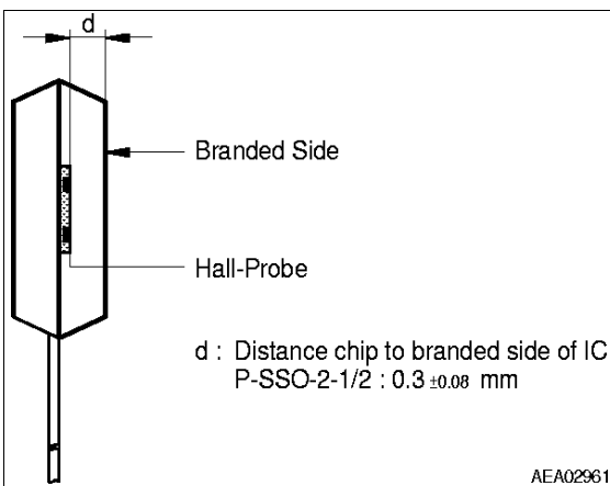
Figure 4-2 Package Outline
