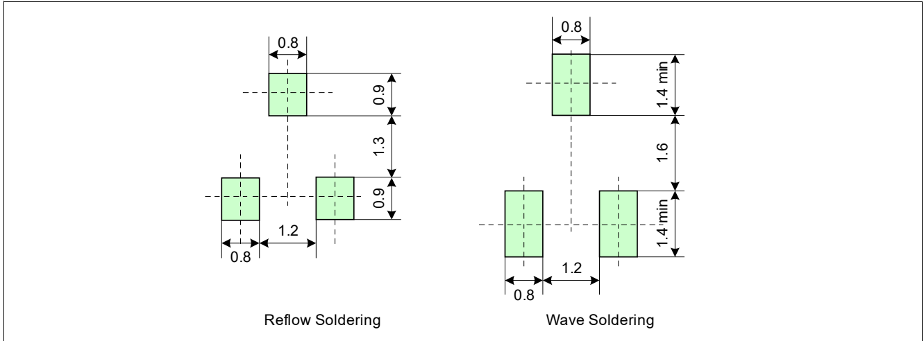
Figure 13 Footprint PG-SC59-3-5
