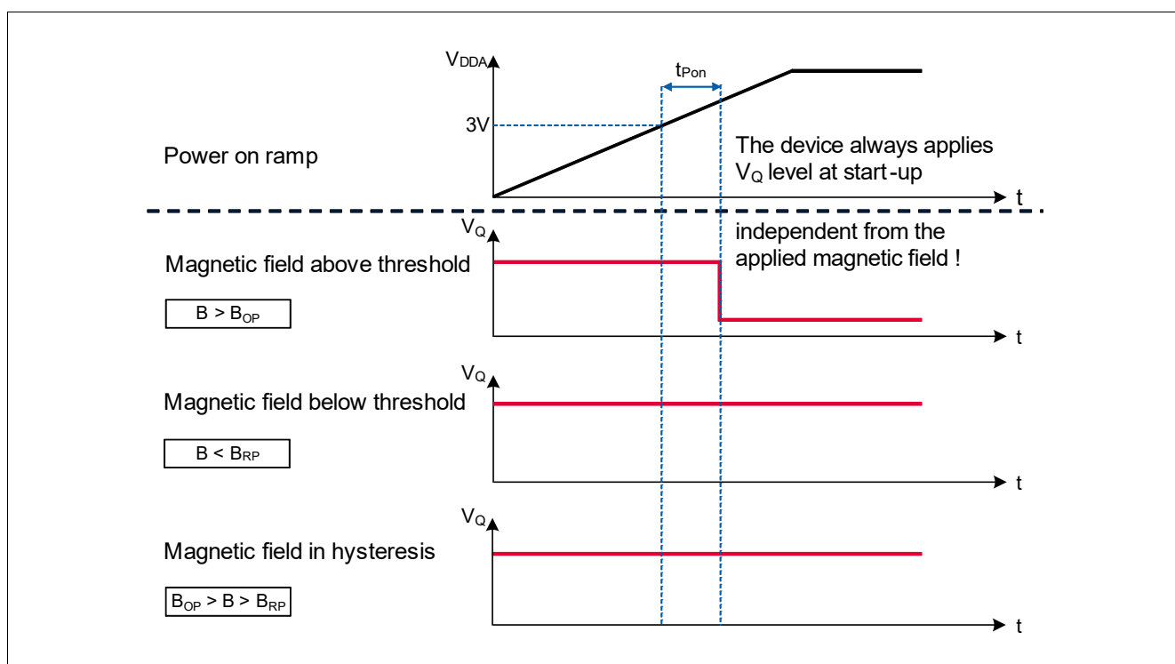
Figure 6 Start-up behavior of the TLE4964-1K
