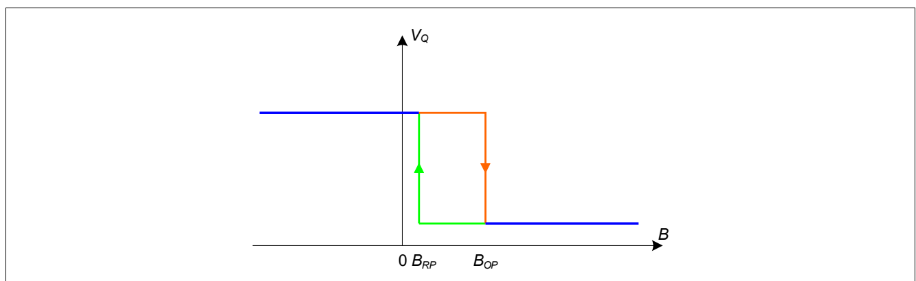
Figure 5 Output signal TLE4964-5M
