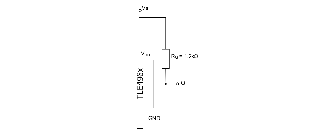
Figure 6 Application circuit #1: only pull-up resistor is necessary
