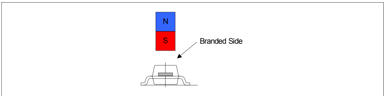
Figure 3-3 Definition of Magnetic Field Direction PG-SOT23-3-15
