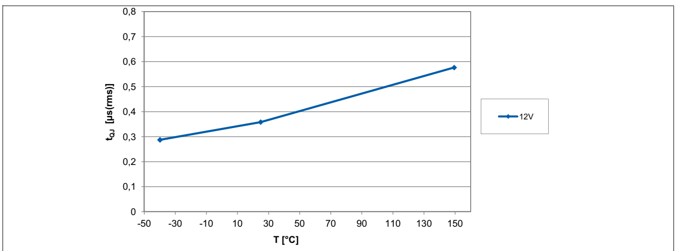
Figure 6-15 Output Signal Jitter of the TLE4968-1M over Temperature
