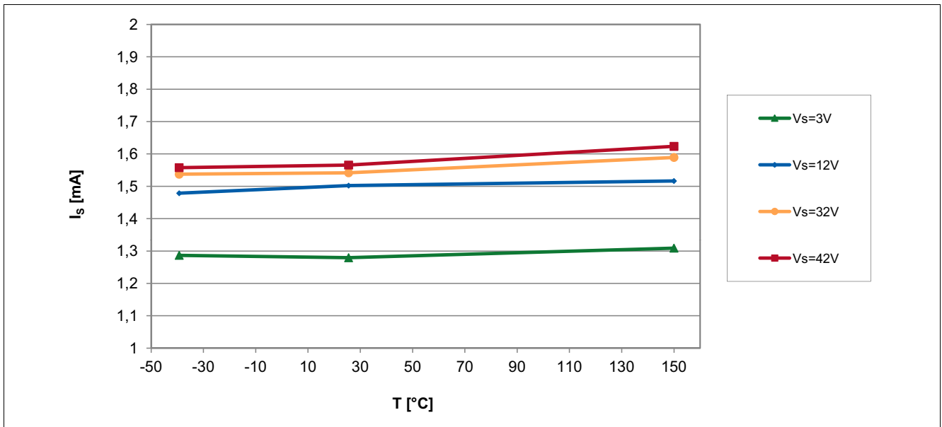
Figure 6-3 Supply Current of the TLE4968-1M over Temperature
