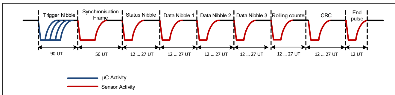
Figure 4 SPC frame with constant trigger length and rolling counter enabled as additional nibble
