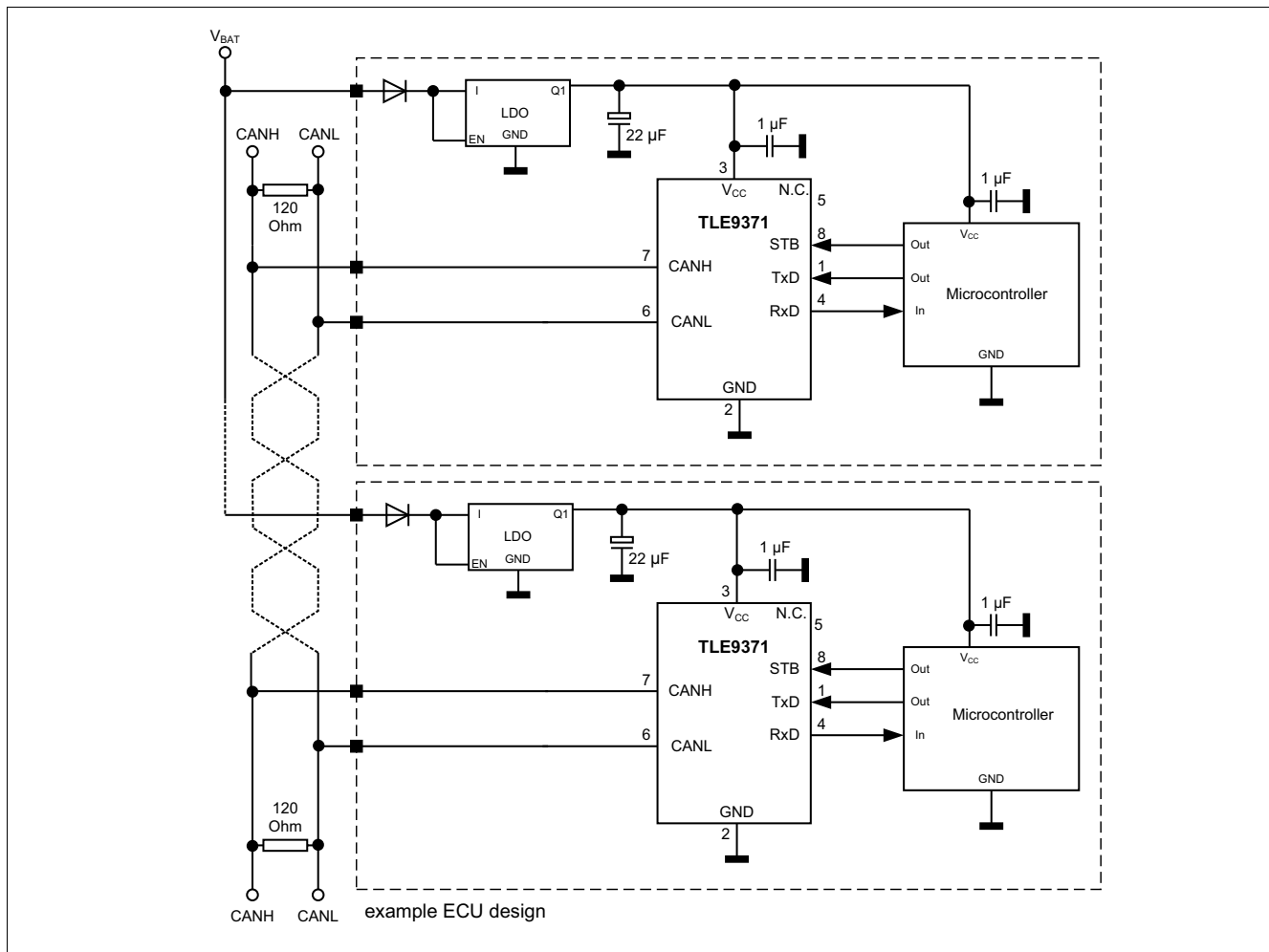
Figure 15 Application diagram
