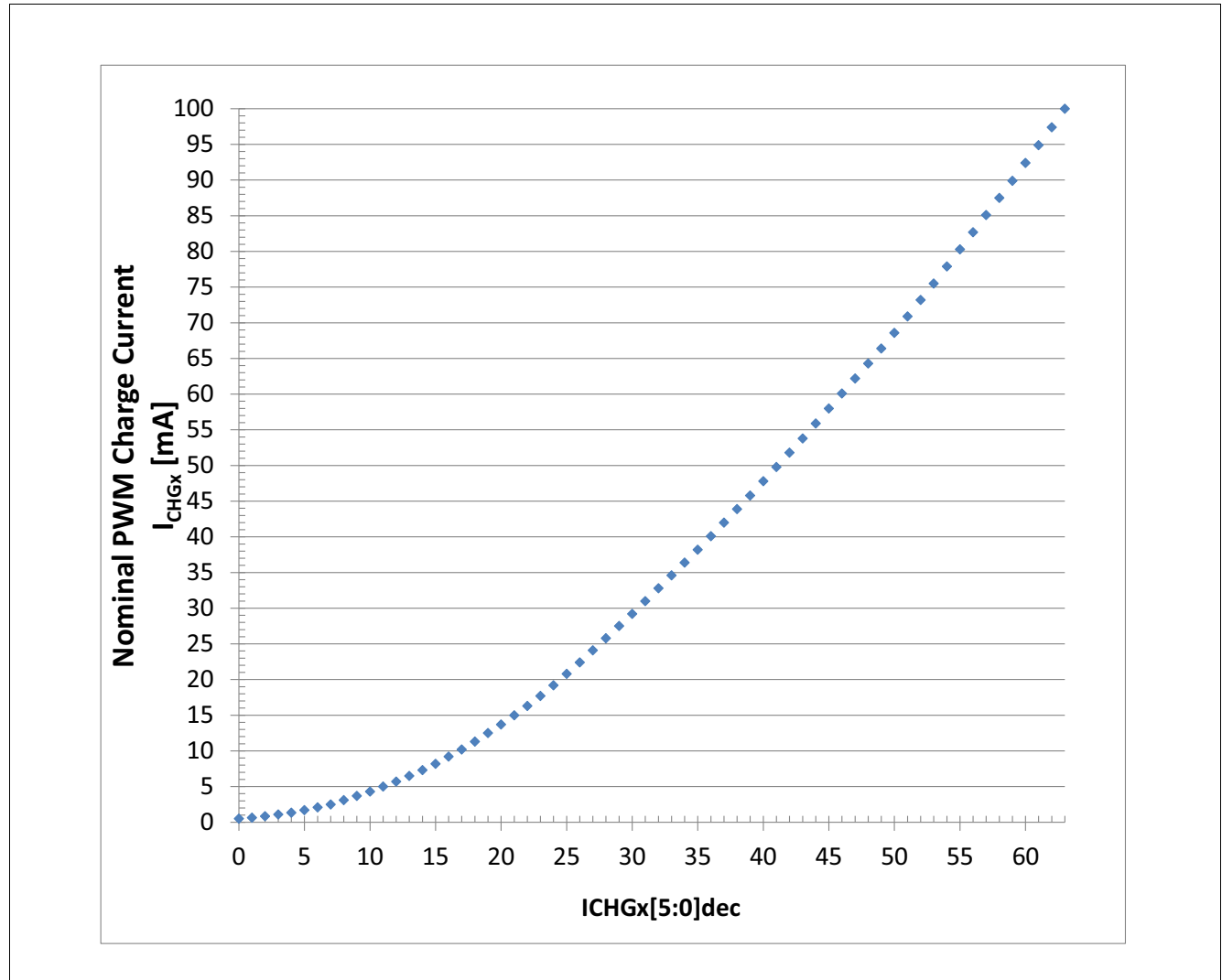
Figure 62 Configurable charge currents in PWM operation
