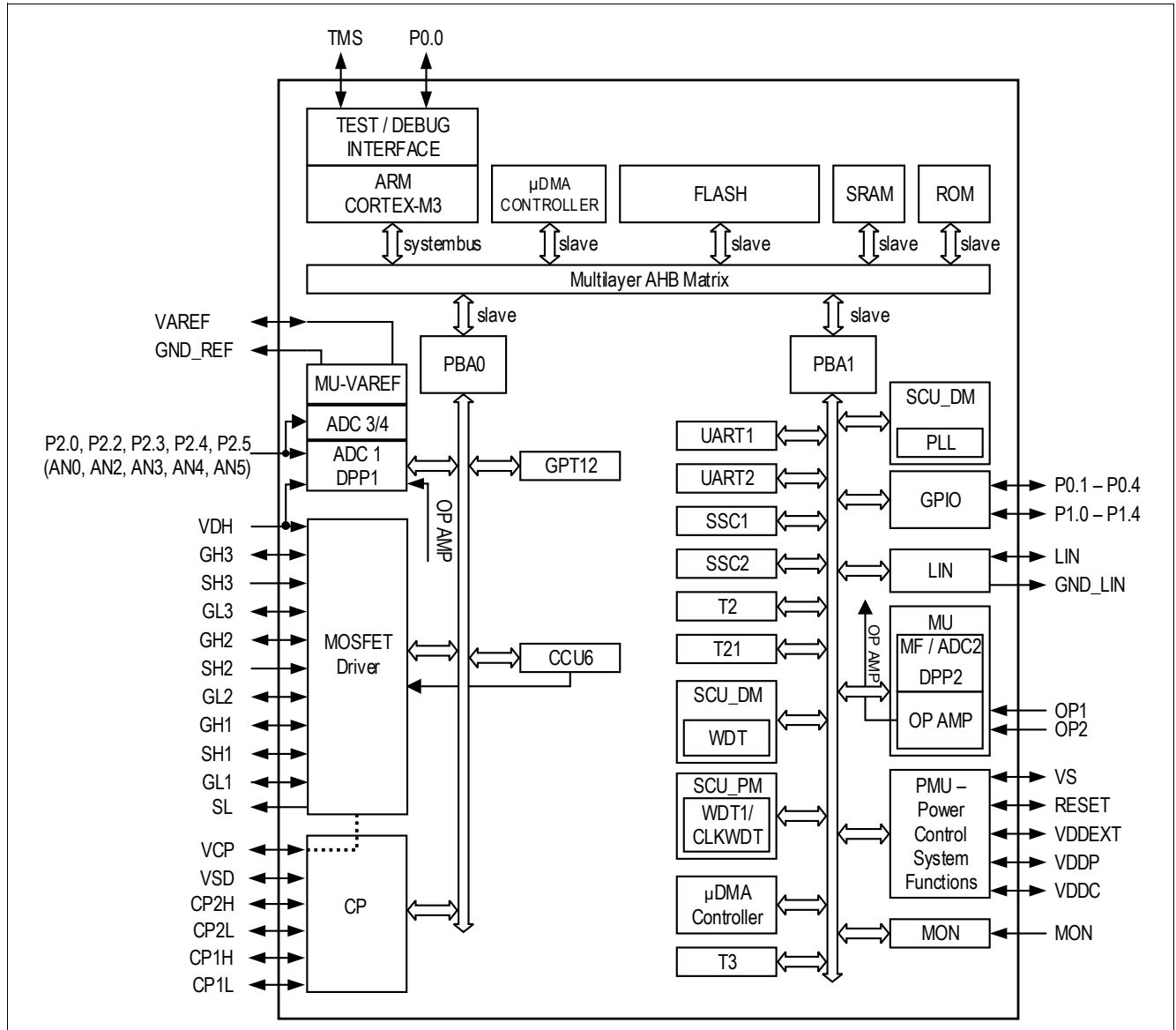
Figure 2 Block Diagram
