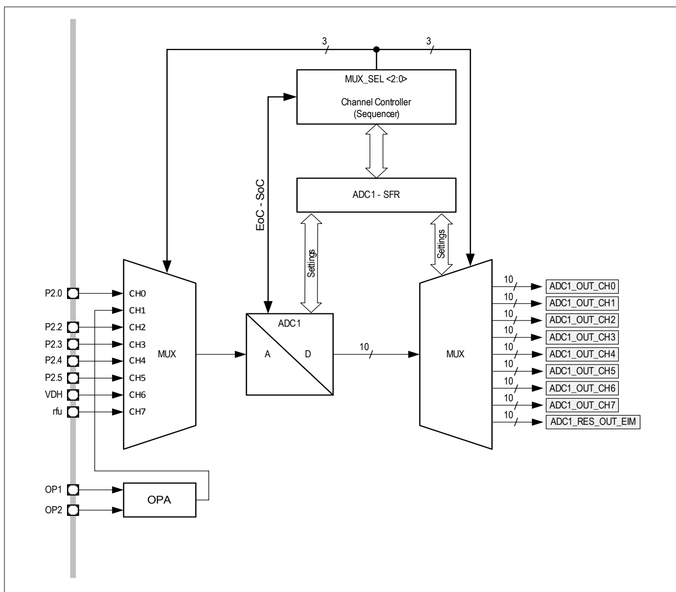
Figure 28 ADC1 Top Level Block Diagram
