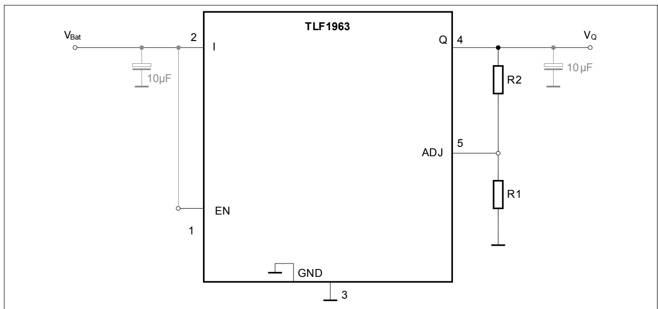
Figure 4 Application Diagram
