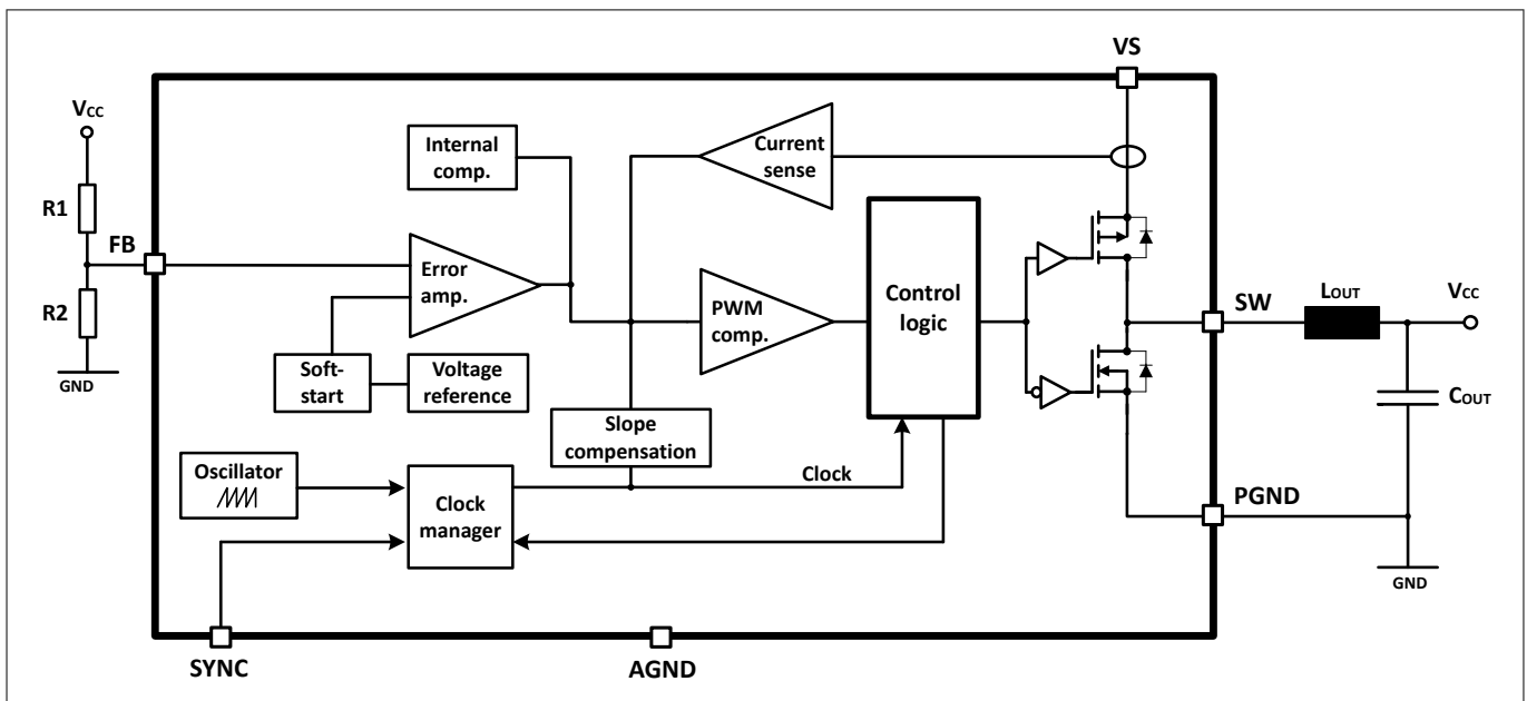
Figure 3 Functional block diagram buck regulator
