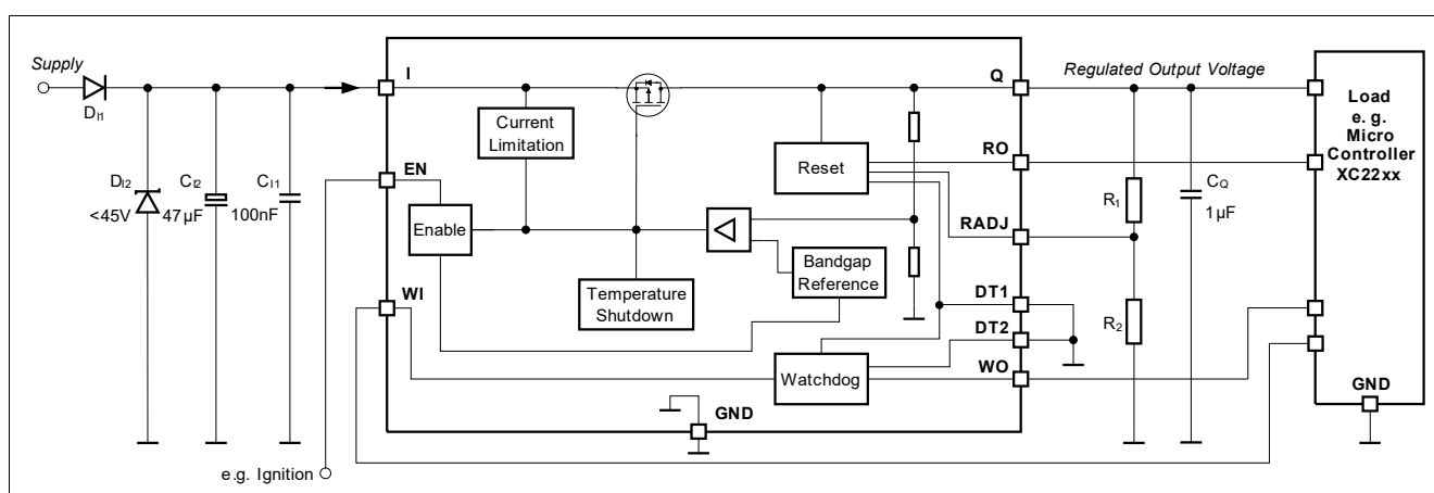
Figure 12 Application diagram
