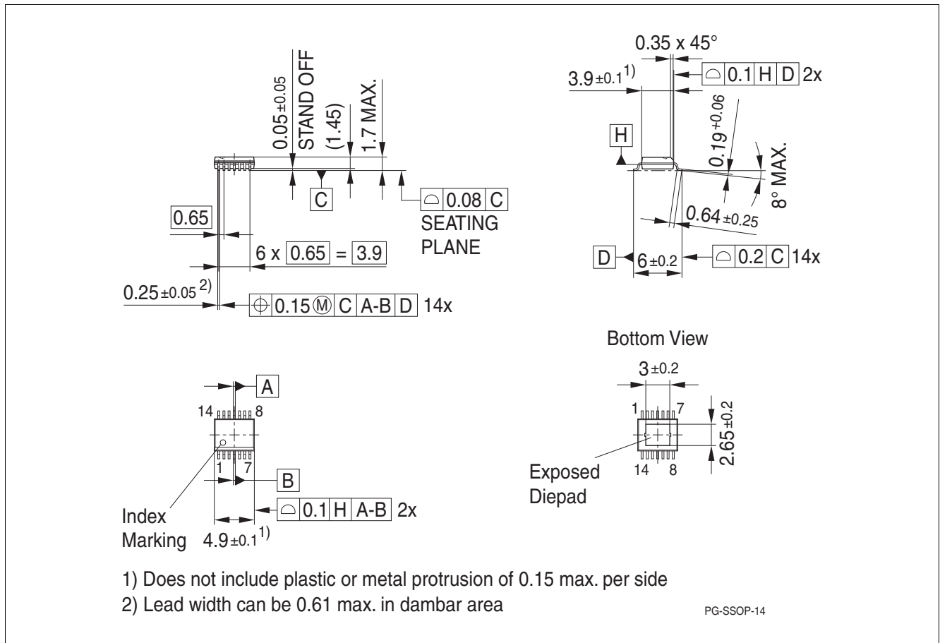
Figure 13 PG-SSOP-14 1)
