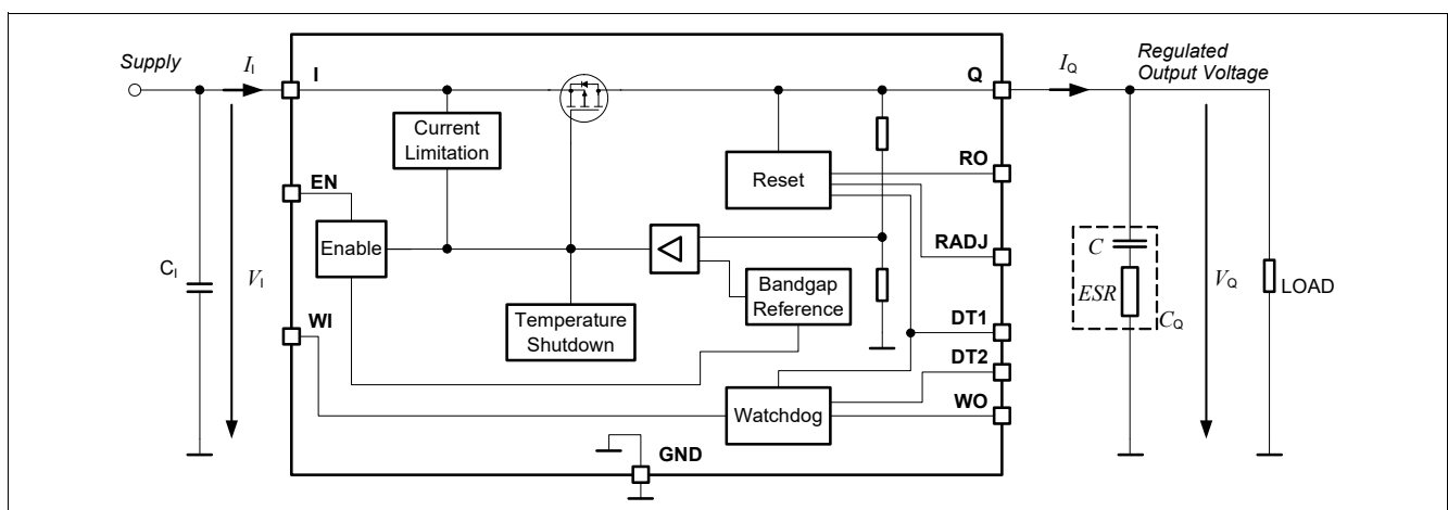
Figure 3 Voltage regulation
