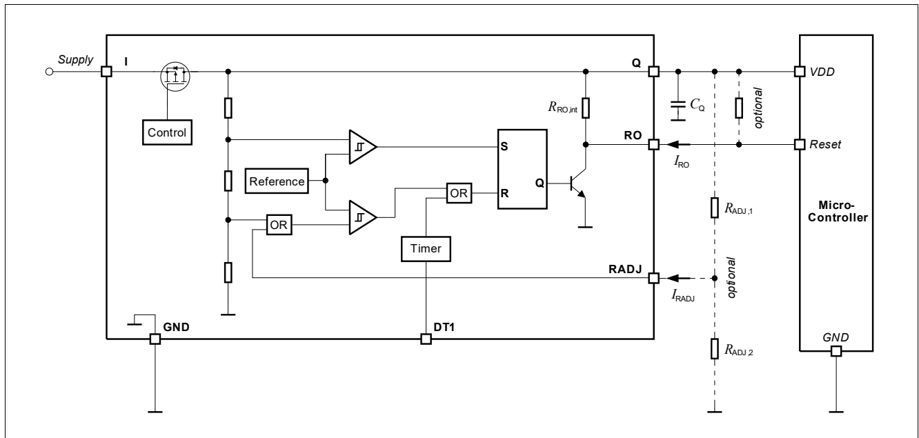
Figure 5 Block diagram reset circuit
