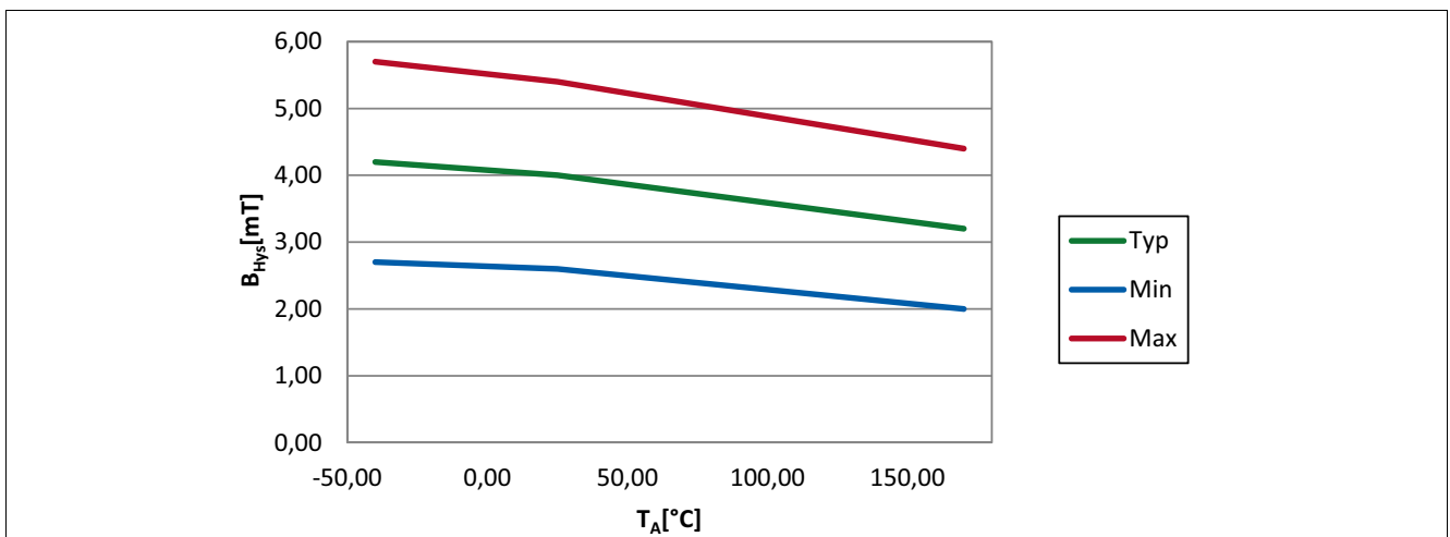
Figure 5-3 Hysteresis (B Hys ) of the TLV4961-1M over Temperature
