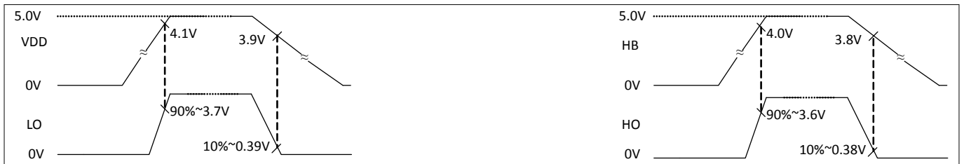
Figure 5 UVLO behavior
