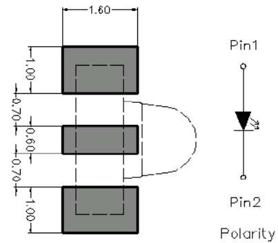
Figure 1. IN-S126ESGHIR Solder Pattern
