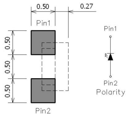
Figure 1. IN-S42DS Solder Pattern
