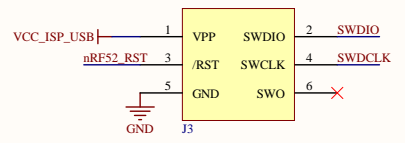
JTAG connector for ISP4520 programming via JTAG Interface
