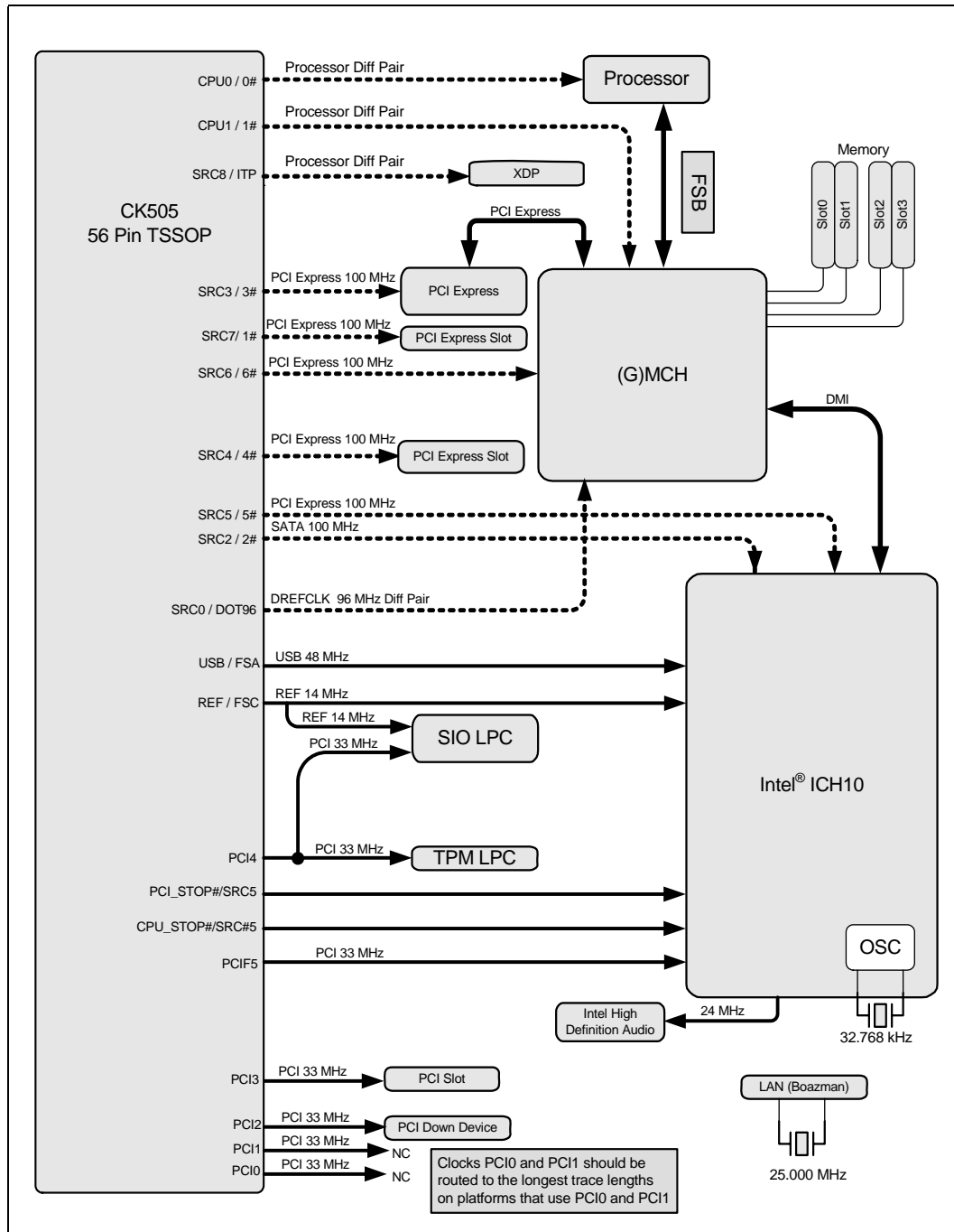
Figure 17. Platform Clocking Diagram
