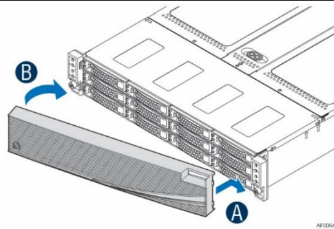
Figure 3. Installing the Front Bezel to the Chassis
