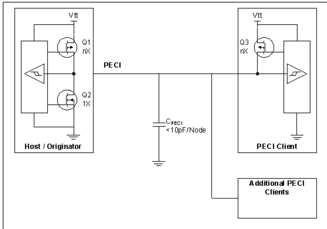
Figure 7-1. Example for PEFI Host-Clients Connection
