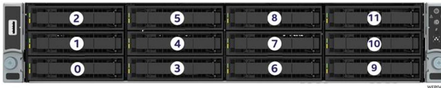
Figure 26. R2312WFxxx SAS/SATA backplane (NVMe* support for drive 10 & 11 only)
