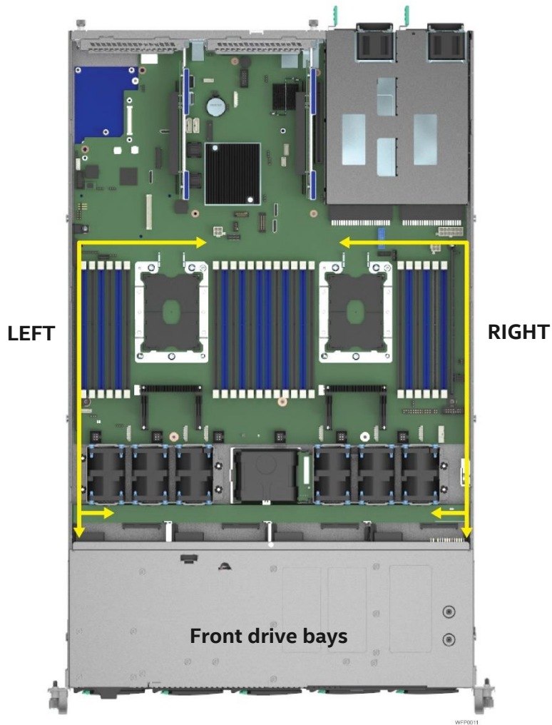
Figure 22. Server system cable routing
