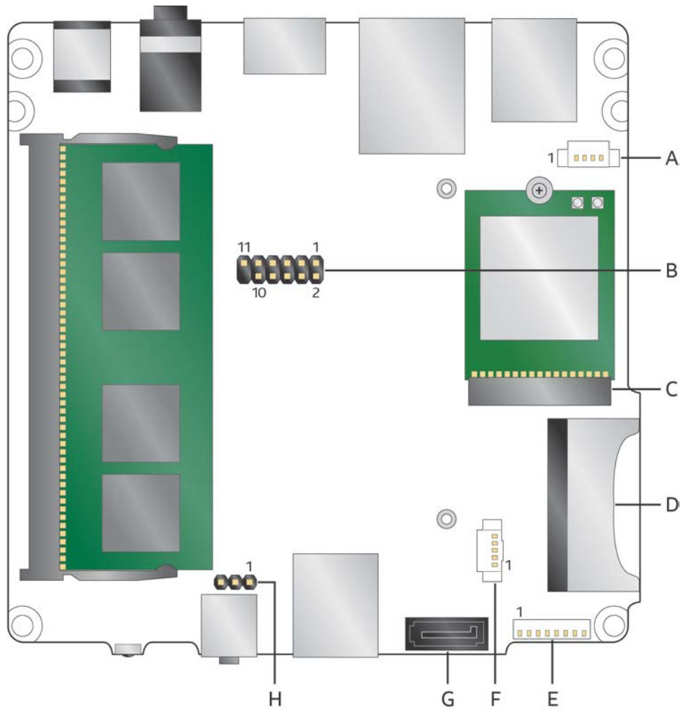
Figure 13. Connectors and Headers (Bottom)
