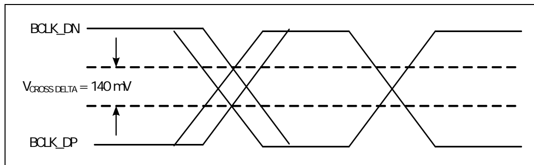
Figure 2-9. BCLK{0/1} Single Ended Clock Measurement Points for Delta Cross Point
