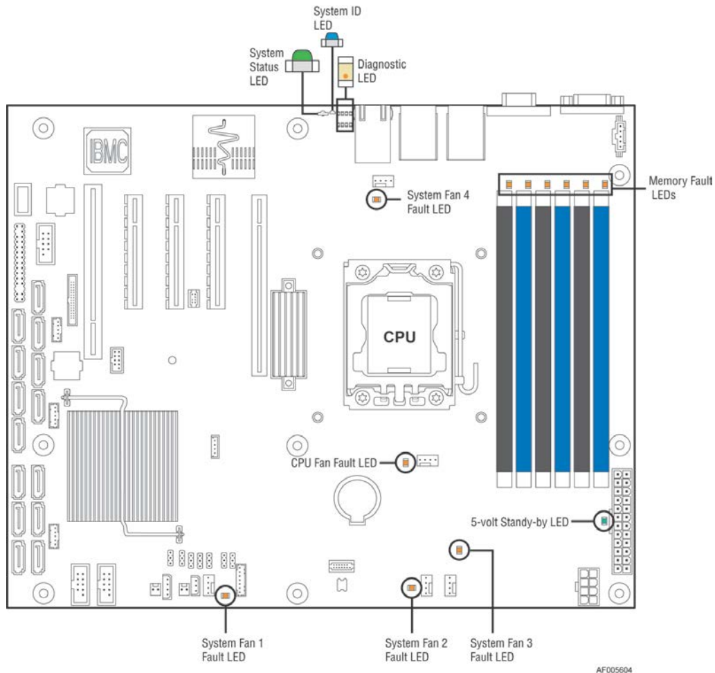
Figure 23. On-Board LED Placement
