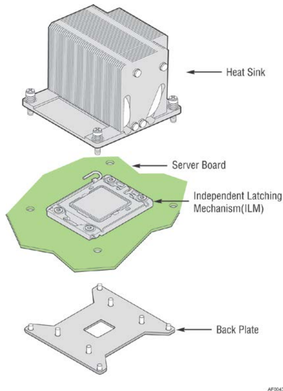
Figure 13. Processor Socket Assembly
