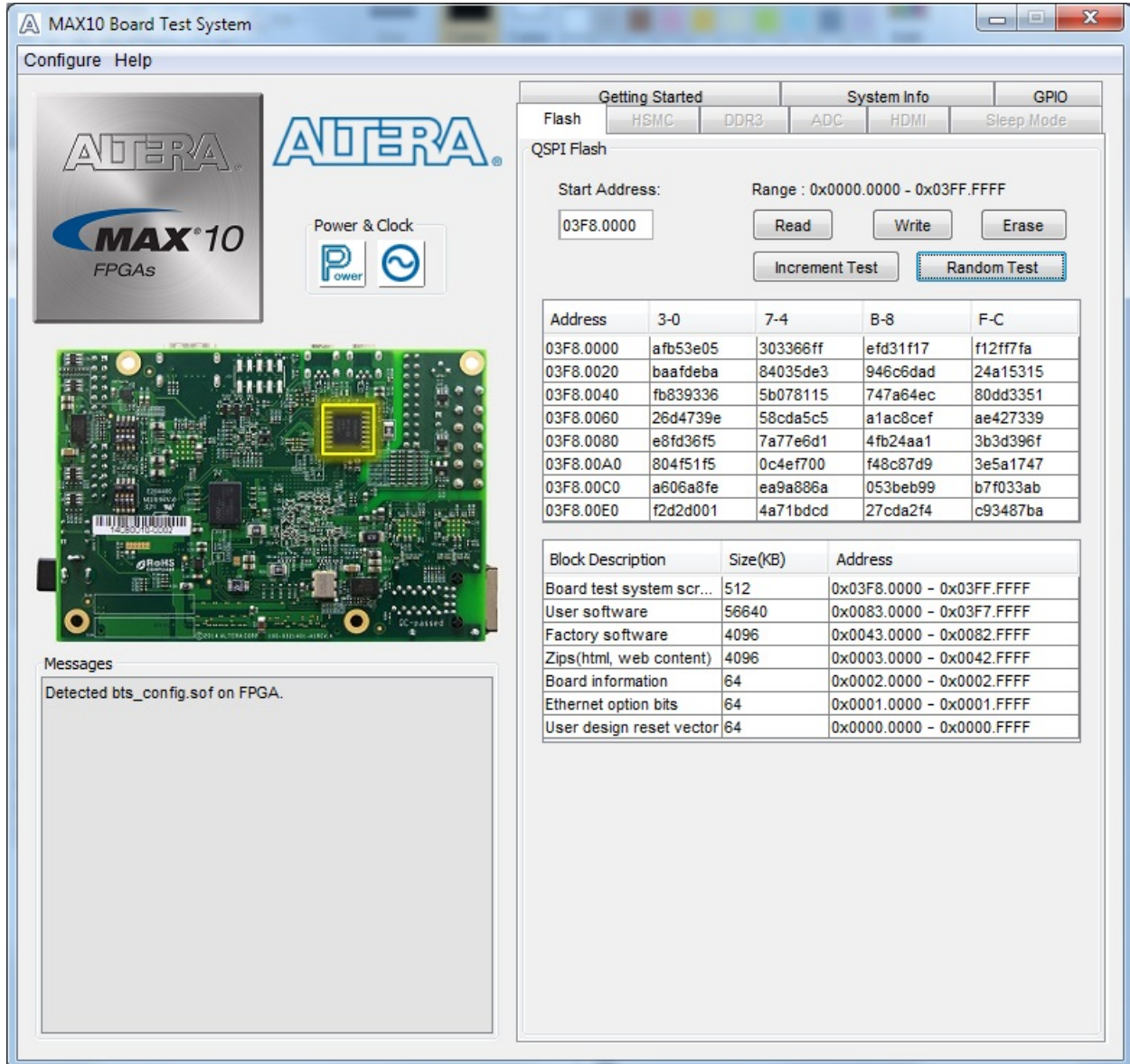
Figure 3-5: The Flash Tab (Detail)
