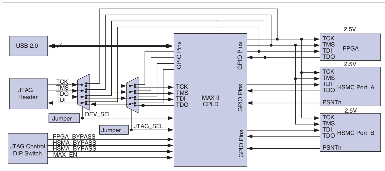
Figure 2-4. JTAG Chain with the MAX II Device and the Cyclone III Device
