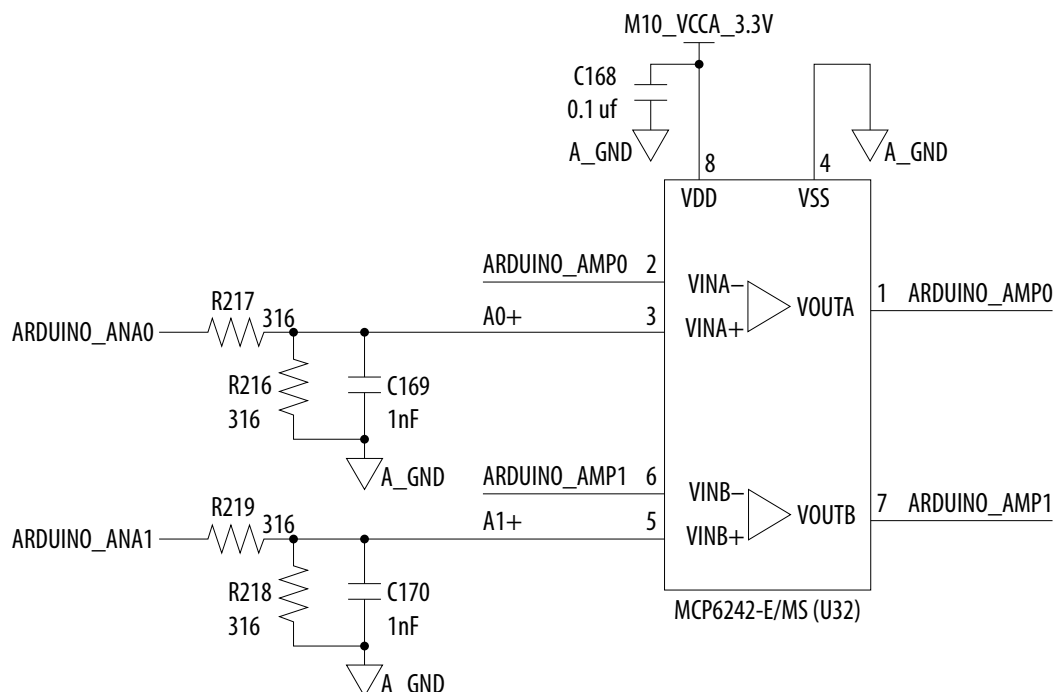
Figure 10. Arduino Analog Input Calculation Example
