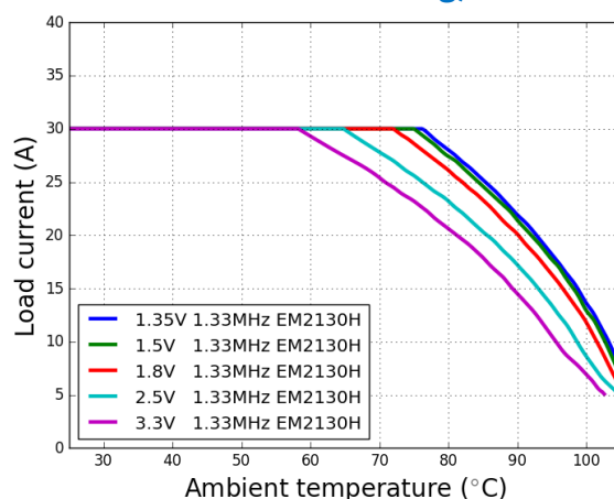
EM2130H Thermal Derating, No Airflow
