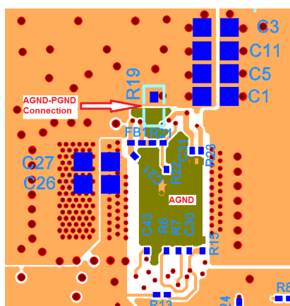
Figure 19: Backside Decoupling
