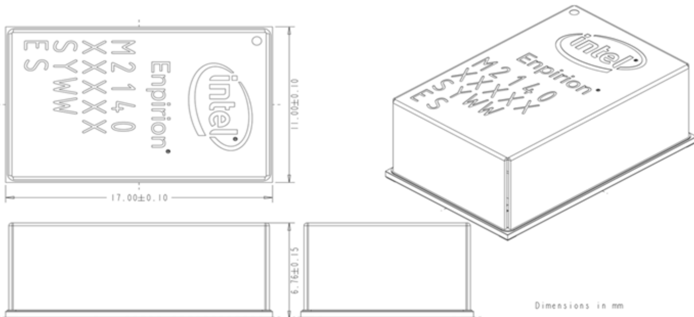
Figure 23: Package Dimensions
