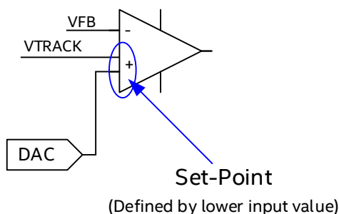
Figure 10: VTRACK Circuitry
