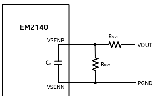
Figure 5: Output Voltage Sense Circuitry
