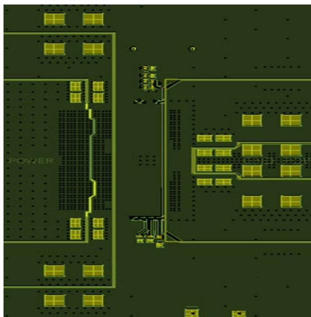
Figure 18: Backside Decoupling
