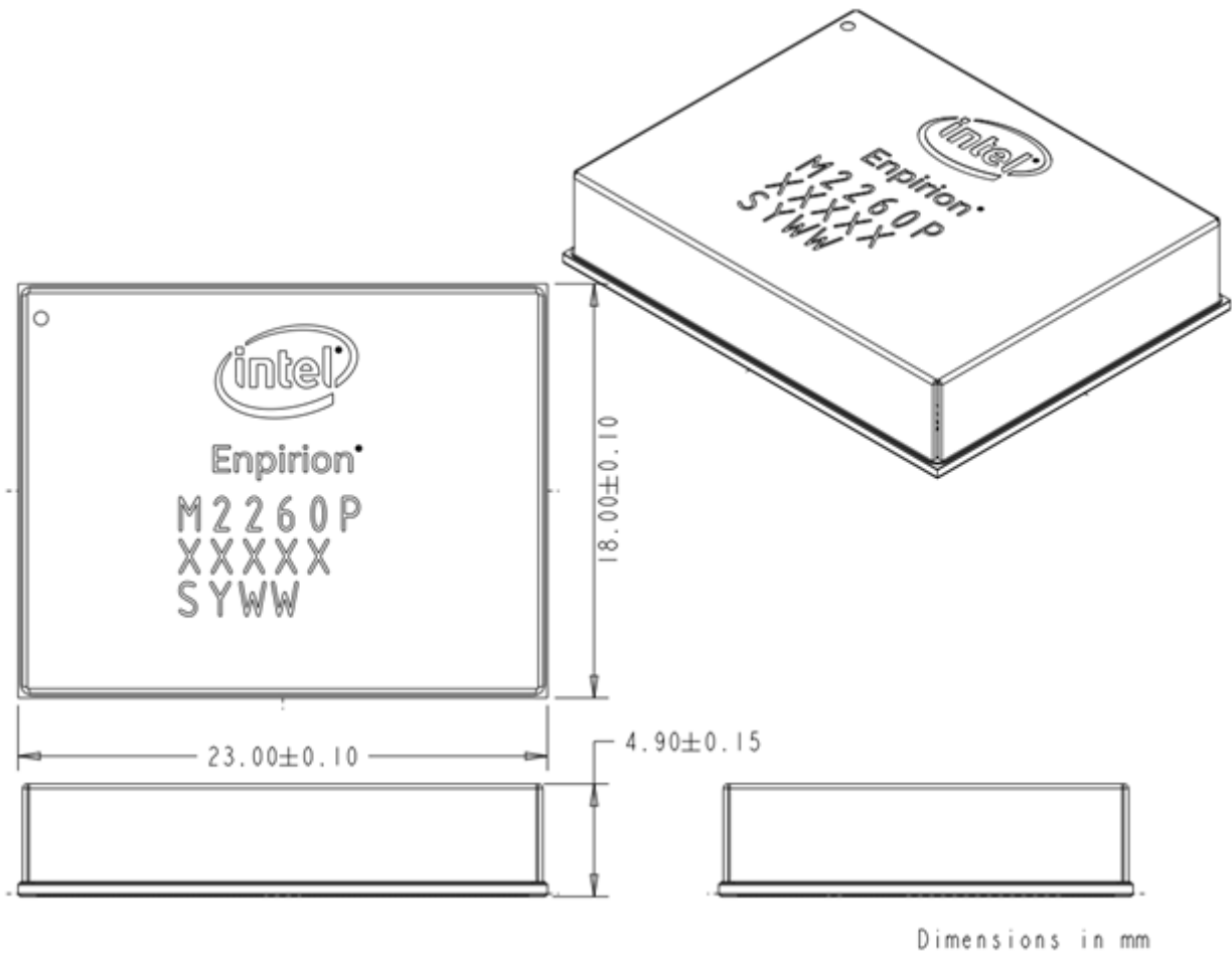
Figure 25: Package Dimensions 1/3
