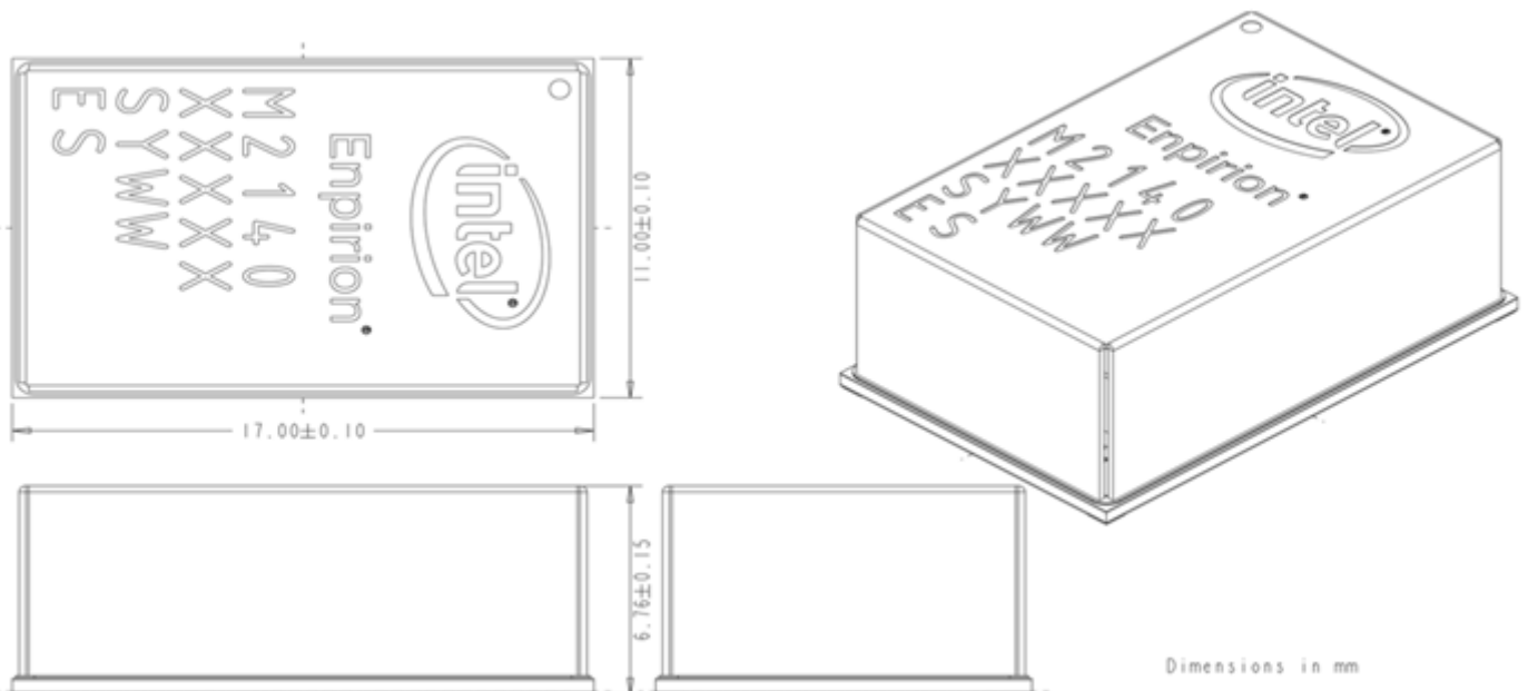
Figure 23: Package Dimensions
