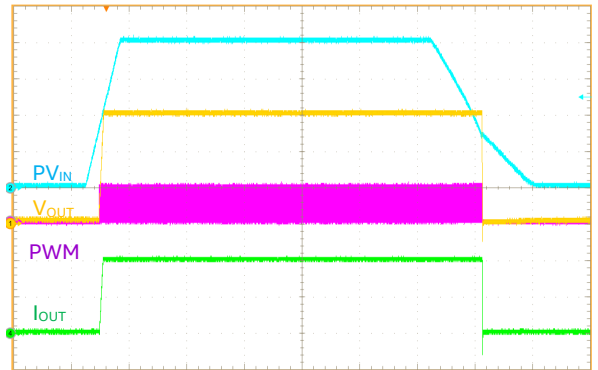
PVIN and PWM: 3 V/div, VOUT: 300 mV/div, IOUT: 20 A/div
