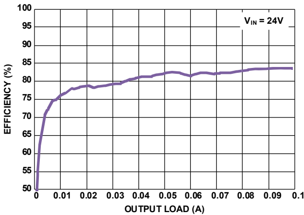
FIGURE 25. EFFICIENCY vs LOAD, PFM, V_{OUT} = 5V
