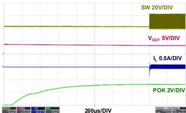
FIGURE 54. NEGATIVE CURRENT LIMIT RECOVERY, PWM
