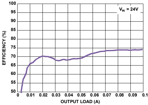
FIGURE 23. EFFICIENCY vs LOAD, PFM, V_{OUT} = 1.8V
