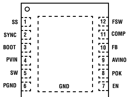
ER3110DI (12 LD 4X3 DFN) TOP VIEW
