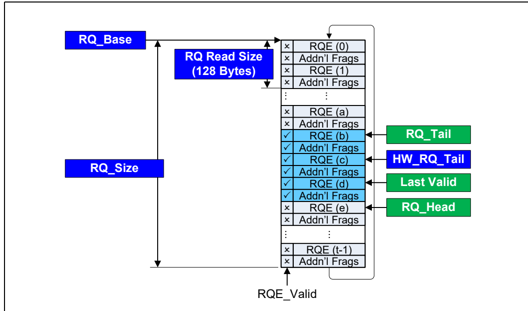
Figure 38-124 shows a typical RQ where software is tracking RQ_head and RQ_Tail and the 10 GbE controller tracks HW_RQ_tail in QP context. Software must size the RQ large enough to support every RQE with the maximum number of additional fragments. All RQEs are shown using two additional fragments and therefore takes 64 bytes. NOP RQEs can be added if necessary to pad RQEs out when necessary to satisfy the RQE alignment requirements. The 32-byte boundary requirements for RQEs means that there is no difference in RQE size between a WR with 2 fragments and a WR with 3 fragments.
