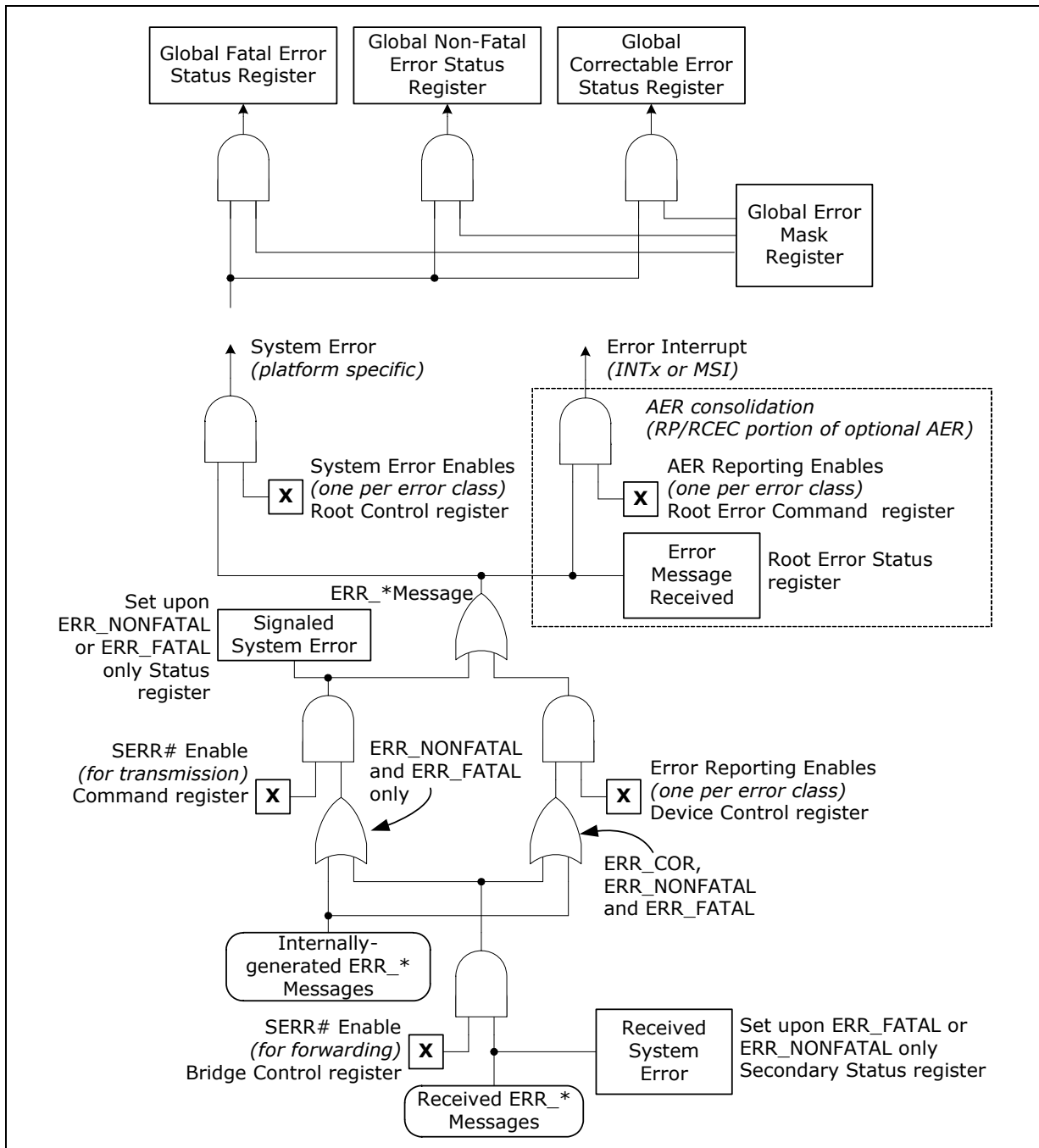
Figure 6-8. PCIe Error Signaling and Logging
