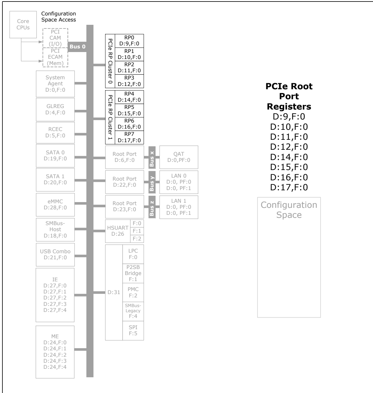
Figure 11-3. Register Map
