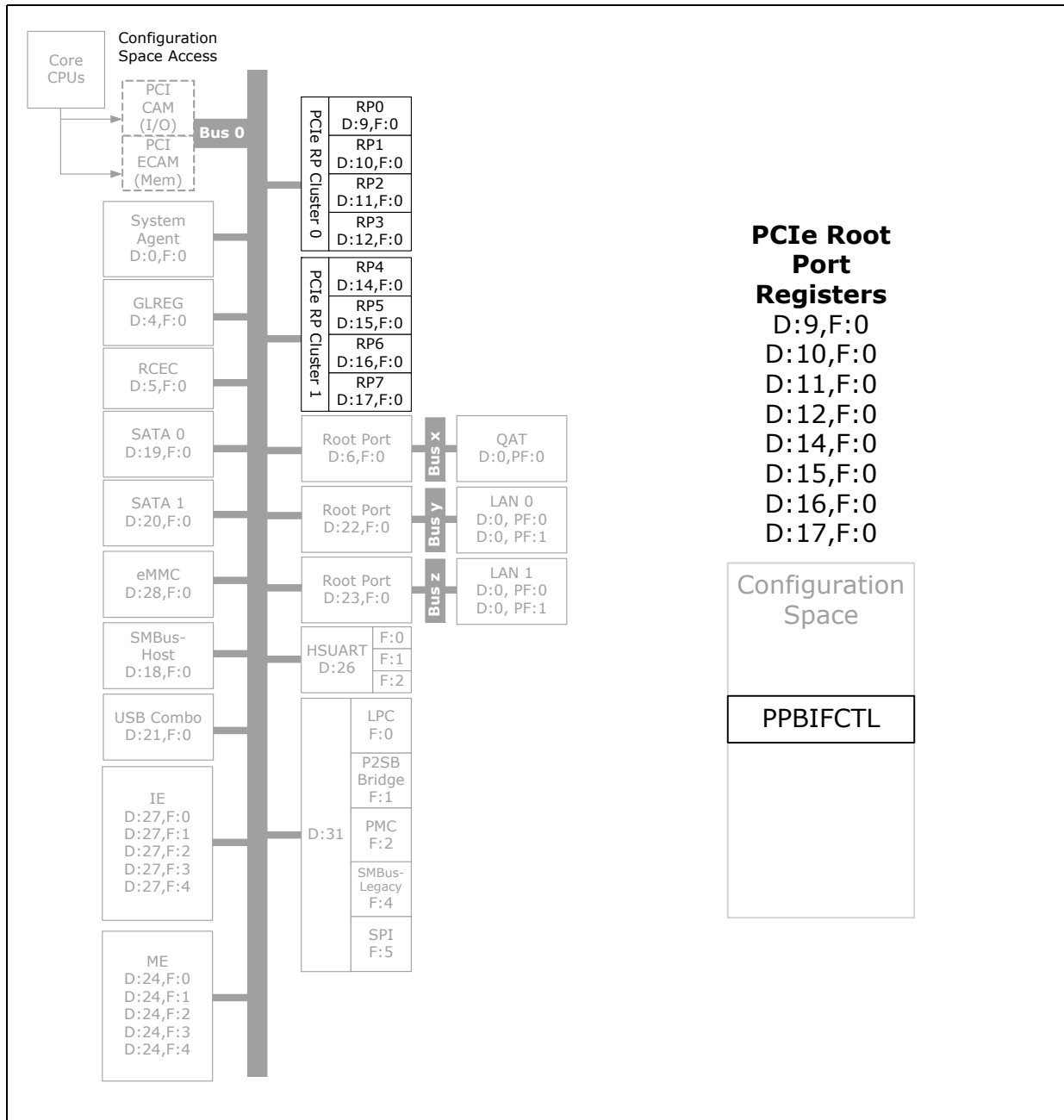
Figure 10-5. Register Map
