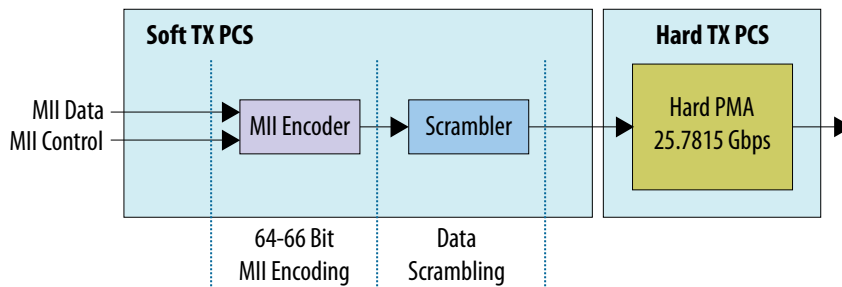
Figure 11. High Level Block Diagram of the Soft TX PCS
