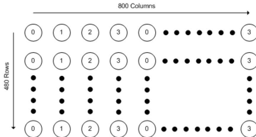
Figure 5–9. Mandelbrot Engine Pixel Interleaving
