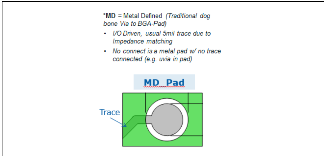
Figure 6-2. Metal-defined pad
