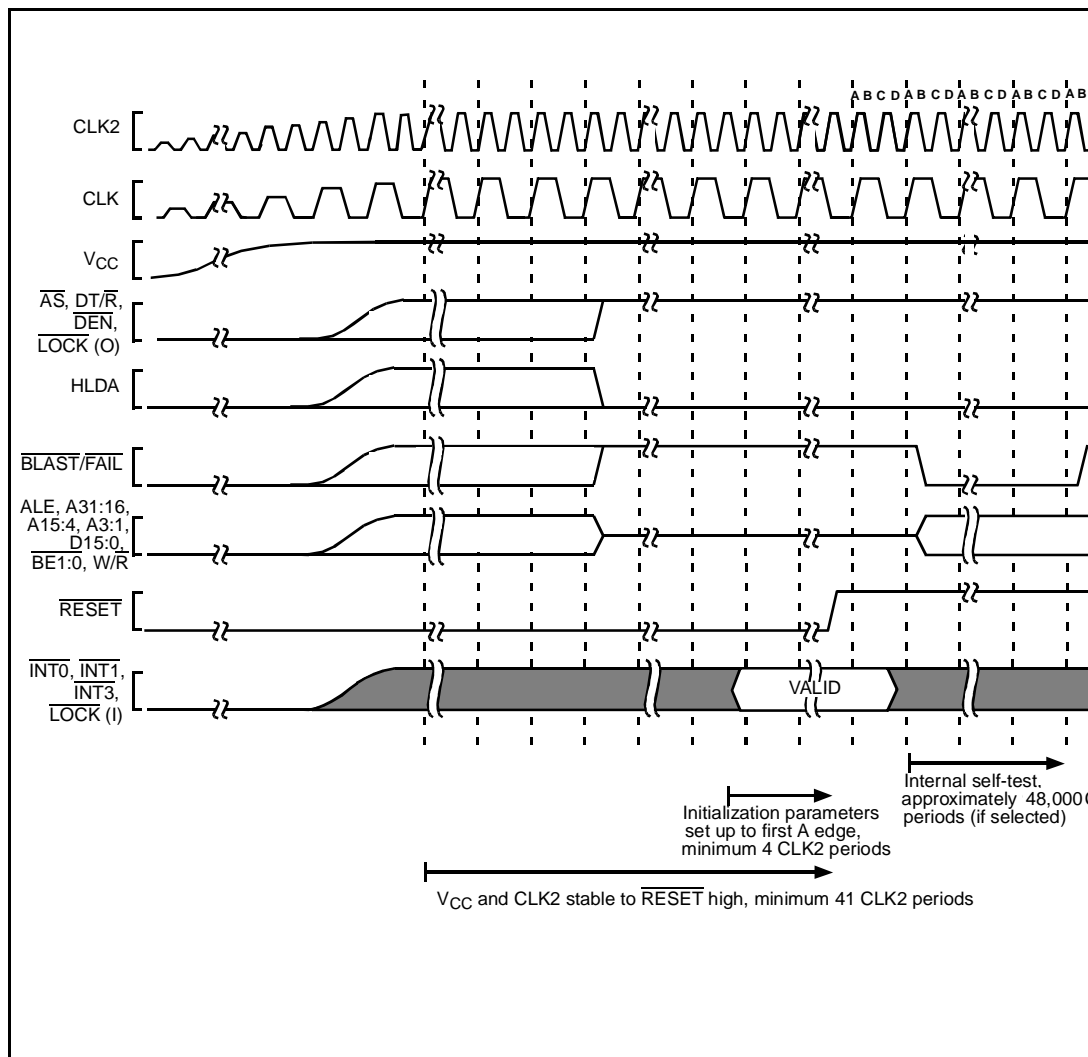
Figure 22. Cold Reset Waveform
