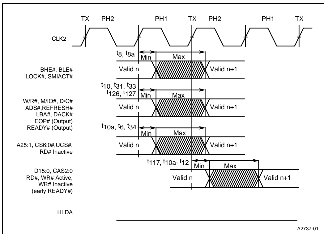
Figure 14. AC Timing Waveforms — Output Valid Delay Timing for External Late READY#
