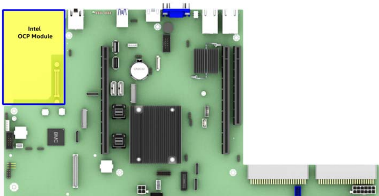
Figure 56. OCP Module Placement
