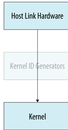
Figure 26. Intel FPGA SDK for OpenCL Offline Compiler-Generated Interface Hardware for a Kernel with the max_global_work_dim(0) Attribute
