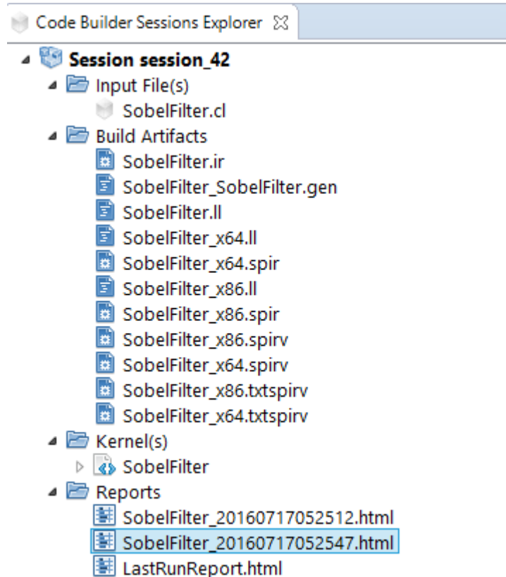
Figure 17. Code Builder Sessions Explorer
