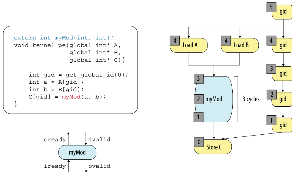
Figure 21. Integration of an RTL Module into an Intel FPGA SDK for OpenCL Pipeline
