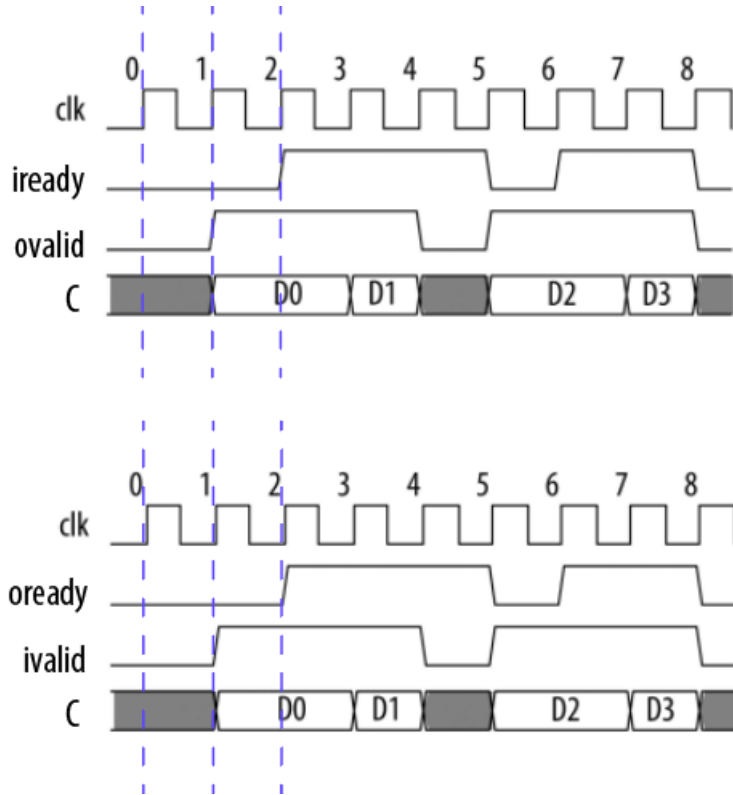
Figure 22. Timing Diagram for Input Data Transfer with Back Pressure
