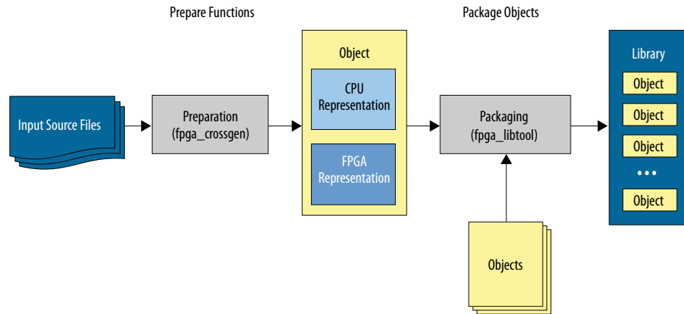
Figure 19. High-level View of the Library Creation Process
