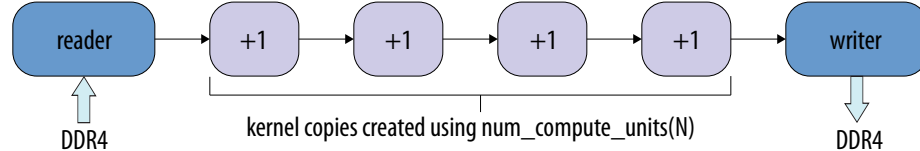
Figure 29. Example Topology of Kernel Copies that Implement Channels
