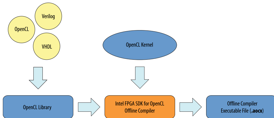
Figure 18. Overview of Intel FPGA SDK for OpenCL's Library Support
