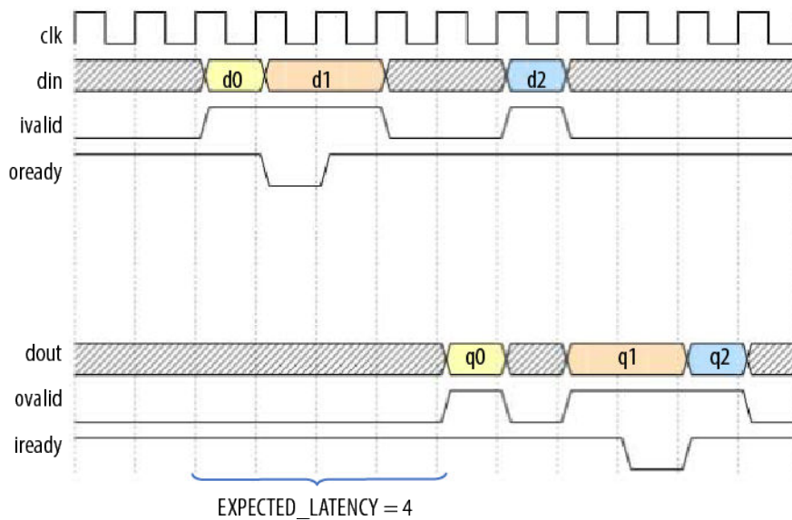
Figure 24. Timing Diagram of a Stallable RTL Component
