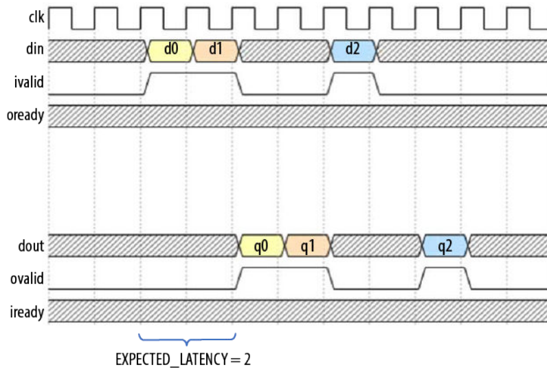
Figure 23. Timing Diagram of a Stall-free RTL Component
