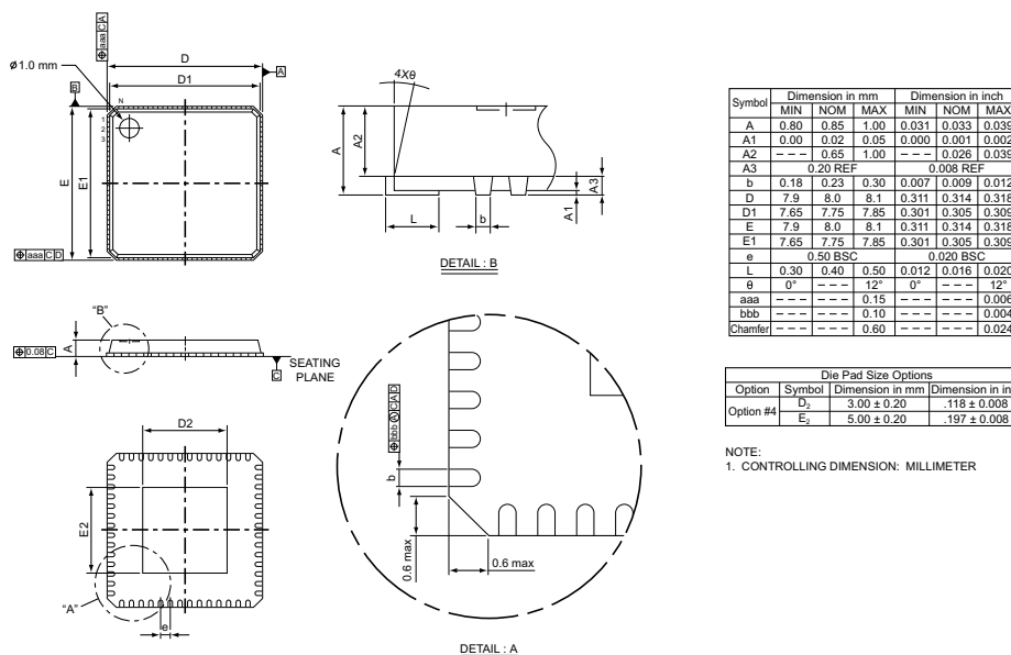
Figure 4. 82567 Mechanical Drawing
